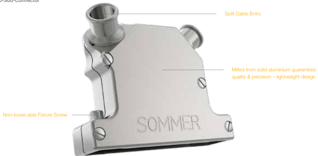
Customized Backshell for D-Sub-Connector
