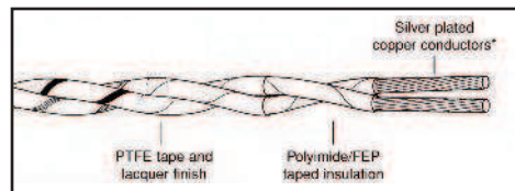
Twisted Single Cores
